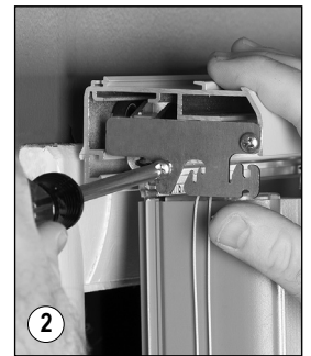
End View - Installation Complete
